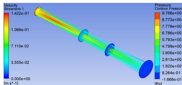
Figure 22: Results of the CFD Simulations for the fluid (Connected). Top left shows fluid traveling through the female part of the valve traveling from the patient (inlet) to the bottom right showing it traveling into the chest drain bottle tube (outlet).
