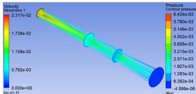
Figure 20: Results of the CFD Simulations for the air flow (Connected). Top left shows air traveling through the female part of the valve traveling from the patient (inlet) to the bottom right showing it traveling into the chest drain bottle tube (outlet).
