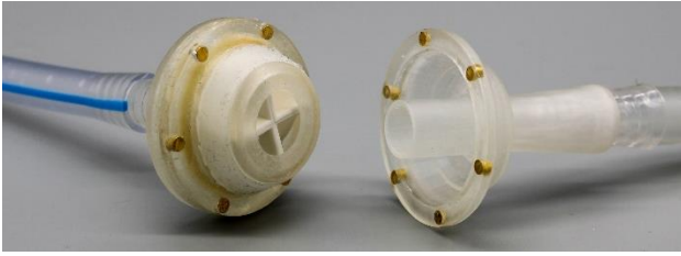
Figure 13: Silicone gasket (left) on break away chest drain valve.
