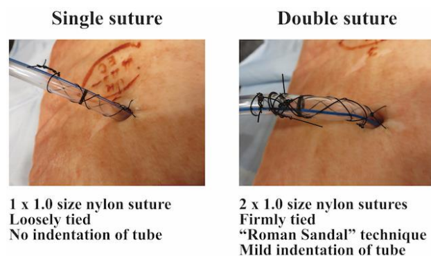
Figure 17: Two methods of chest drain fixation.
