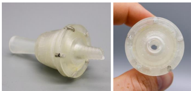
Figure 9 (Left): Initial breakaway chest drain valve concept connected; (Right): showing the one-way valve is fully open and created uninterrupted flow.
