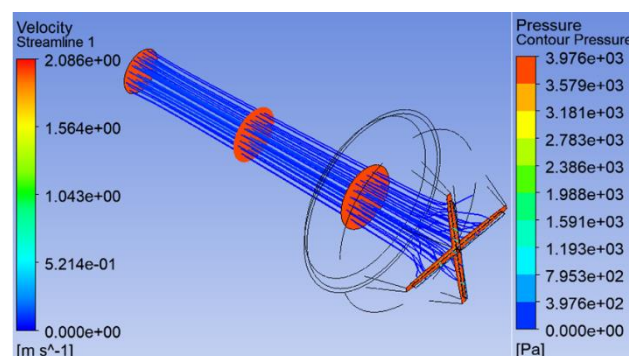
Figure 23: Results of the CFD Simulations for the fluid (Disconnected). Top left shows fluid traveling through the female part of the valve traveling from the patient (inlet) to the bottom right showing it traveling out of the cross-slit valve (outlet).
