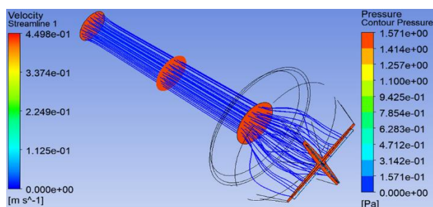
Figure 21: Results of the CFD Simulations for the air flow (Disconnected). Top left shows air traveling through the female part of the valve traveling from the patient (inlet) to the bottom right showing it traveling out of the cross-slit valve (outlet).
