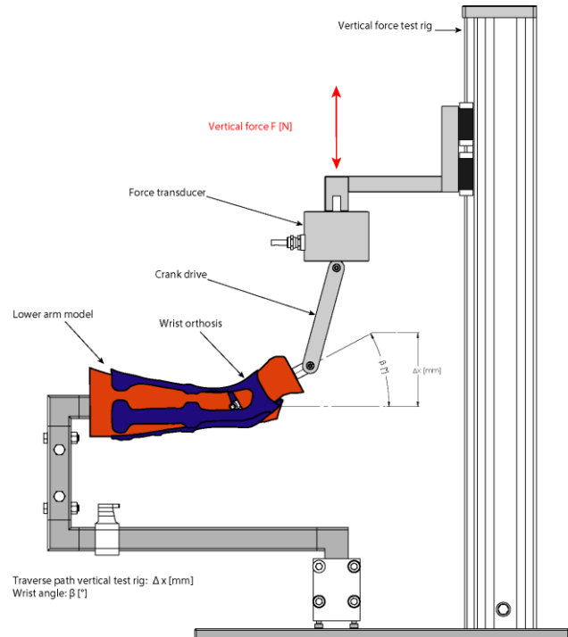
Figure 4: Schematic set-up of the test rig for wrist hand orthoses (WHOs).
