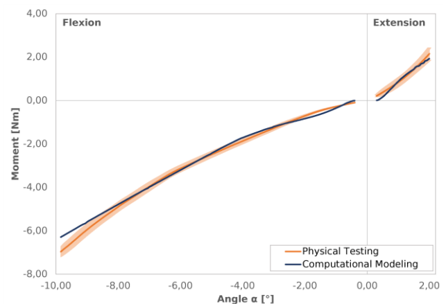
Figure 6: Comparison of the moment-angle characteristic curve between simulation and experimental data. The pale orange area around the curve shows the coefficient of variation for the experimental data.
