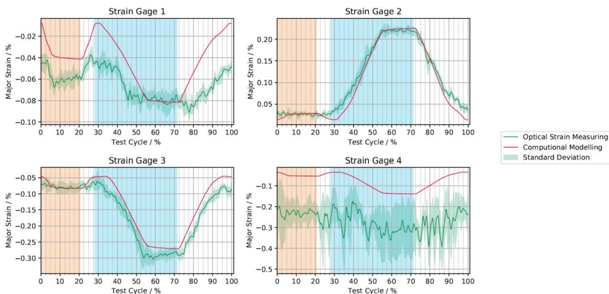
Figure 8: Representation of the major strain characteristic depending on the test cycle for strain gage 1 to 4, respectively. Compared are the results of the non-contact optical measurement system (green) with the computational model (red). The colored area around the curve represents the standard deviation. The load phase in extension (orange) and in flexion (light blue) is highlighted in color, whereas the release phase is shown in white.
