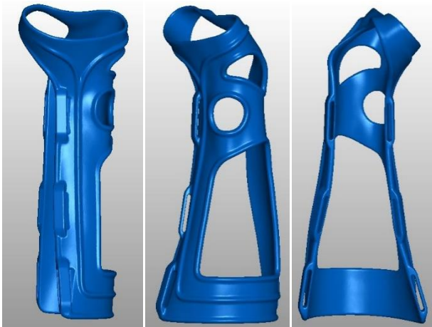
Figure 1: Dorsal (left), ulnar (middle), and radial (right) view of the custom-made 3D printed wrist hand orthosis (WHO), designed by Care Center Deutschland GmbH.
