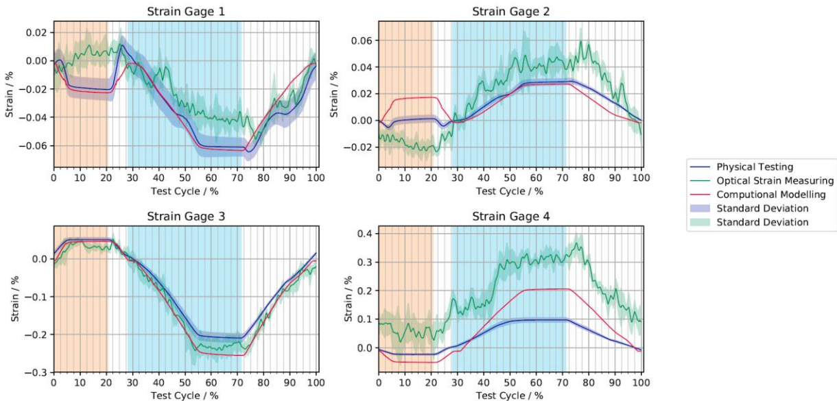
Figure 7: Representation of the characteristic curve of the strains depending on the test cycle for strain gage 1 to 4, respectively. Compared are the results of the strain gages (blue), the non-contact optical measurement system (green), and the computational model (red). The colored area around the curve represents the standard deviation. The load phase in extension (orange) and in flexion (light blue) is highlighted in color, whereas the release phase is shown in white.
