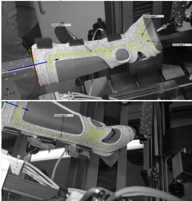
Figure 5: Positioning of the strain gages on the 3D printed WHO to validate the occurring strains.
