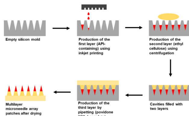
Figure 2: Manufacturing process of multilayer MAPs using inkjet printing and centrifugation
