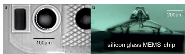
Figure 4: Micronozzle printed on chip: (a) View from above of the nozzle during the printing process. The rectangular roots and the circular sealing structures are visible. (b) An optical microscope image of a printed nozzle on the MEMS chip (side view). The nozzle is 850 \mu\text{m} wide, 350 \mu\text{m} high, and 310 \mu\text{m} deep.
