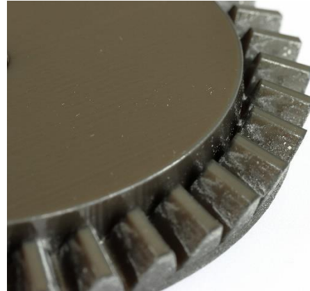
Figure 3: Contact pattern on the gear in drag direction shows a concentration of wearout along the upper half of the teeth only towards the smaller radii.
