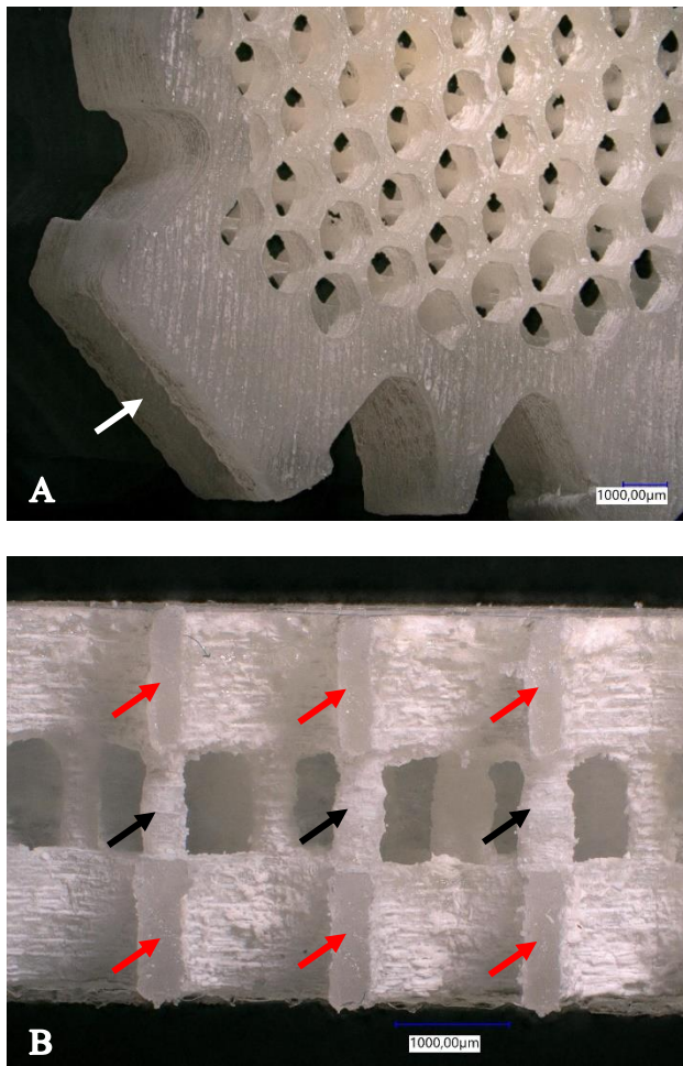
Figure 4: Insights of the fabricated mMS. (A) Tilted view under an angle of 35°. White arrow indicates the inlet of the fluidic channel. (B) Cross section of the mMS. Black arrows indicate the support structures. Red arrows indicate the cross section of the honeycomb sidewalls.
