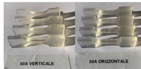
Figure 1: Tensile test specimen.
