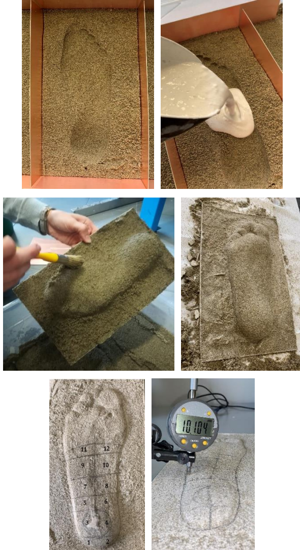
Figure 7: Sequence of the fabrication of the footprint mold, followed by the schematics of the foot region map and the mold characterization to measure the local height of the footprint.
