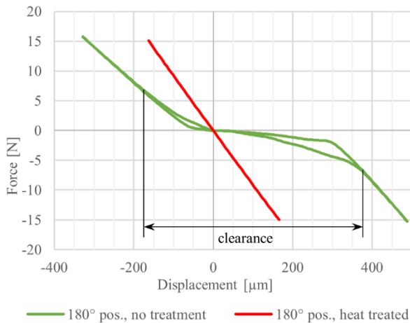
Figure 4: Force displacement curves to determine the clearance of the joints, 500 \mu\text{m} circumferential design clearance [7]
