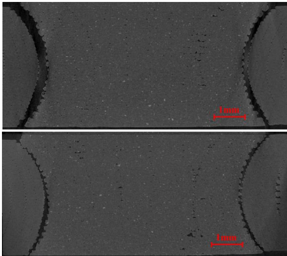
Figure 5: Micro-CT scans of two joints before the heat treatment, top: 500 \mu\text{m} circumferential design clearance; bottom: 300 \mu\text{m} circumferential design clearance [7]
