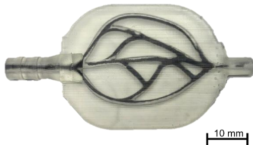
Figure 4: Embolization module 1.6 mm vessel diameter after the treatment simulation with Onyx (black)
