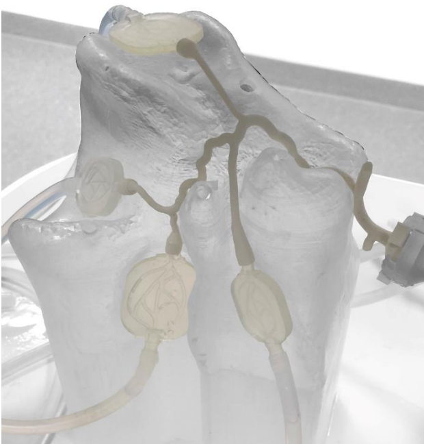
Figure 2: Setup of the cSDH treatment simulation in the HANNES simulator with the MMA model and the integrated embolization modules
