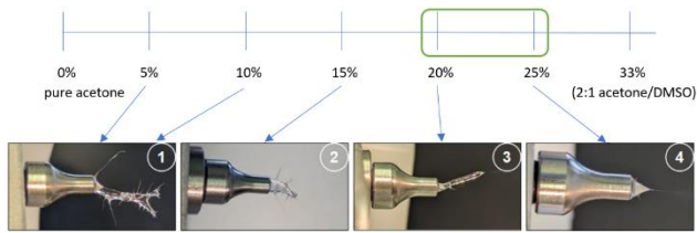
Figure 2: Taylor cone behavior for selected acetone/DMSO compositions.
