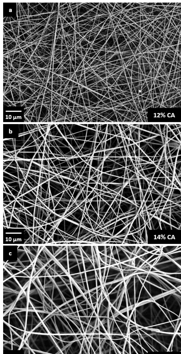
Figure 3: SEM images of cellulose acetate mesh with a polymer content of 12% (a), 14% (b) and 16% (c) (w/v).
