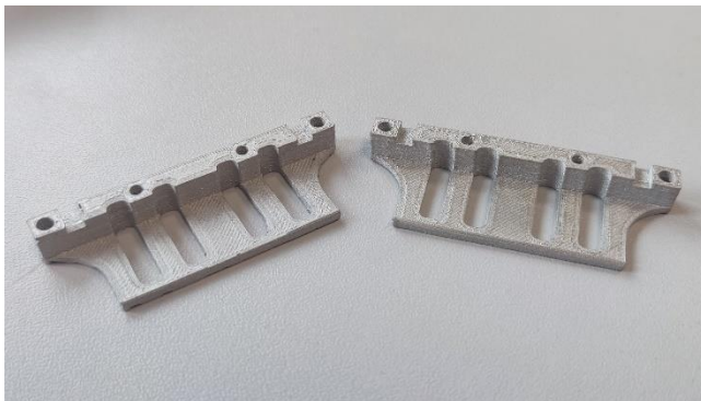
Figure 5: Metal MEX manufactured sensor parts after the sintering process
